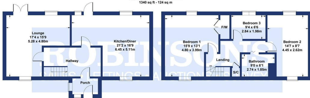
GROUND FLOOR
